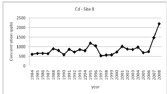
Figure 5. Cadmium concentrations in Narmak
