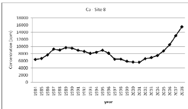
Figure 8. Calcium concentrations in Narmak
