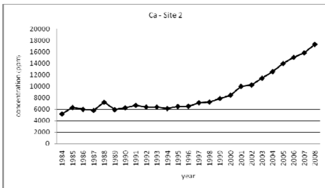
Figure 7. Calcium concentrations in Saadatabd
