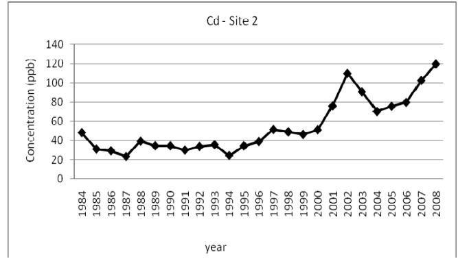
Figure 3. Cadmium concentrations in Saadatabad
